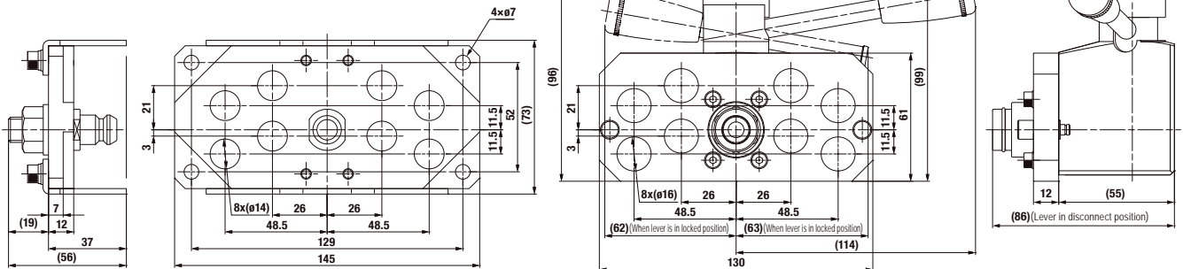
Plate model of Plug side MAM-B-1P8-CL
