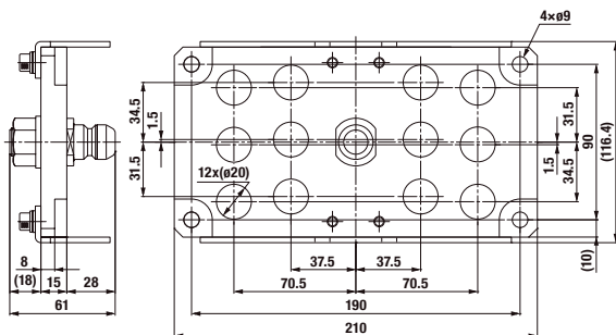
Plate model of Plug side MAM-A-3P12-CL
