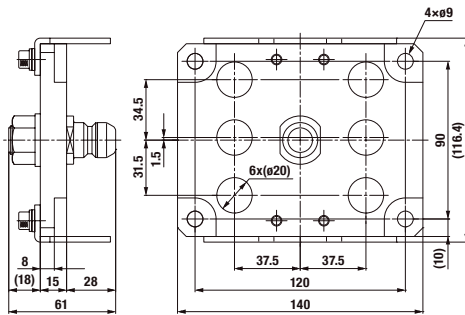
Plate model of Plug side MAM-A-3P6-CL
